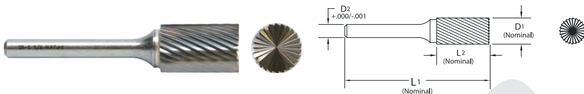
3mm Shank Burrs (Standard Length)
