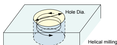
Helical milling
