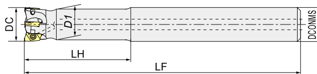
Fig.1 (Standard type)
