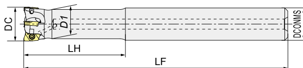
Fig.2 (Undercut type)
